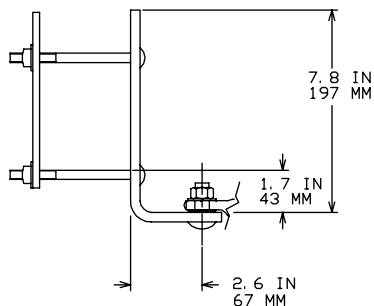
NEMA "B" BRACKET
